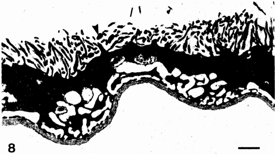
Fig. 8. A higher magnification electron micrograph of the epithelium in the storage region. Some of the microvilli contain mitochondria (arrowhead). l , lumen. Scale bar, 1 \mu\text{m} .
