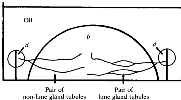
Fig. 1. Diagram of the in vitro Malpighian tubule assay system for determining calcium accumulation rates. Excised tubule pairs are suspended in a saline bathing droplet ( b ) isolated under mineral oil. The cut ends of the tubules are pulled out and allowed to secrete droplets ( d ) onto glass posts.
