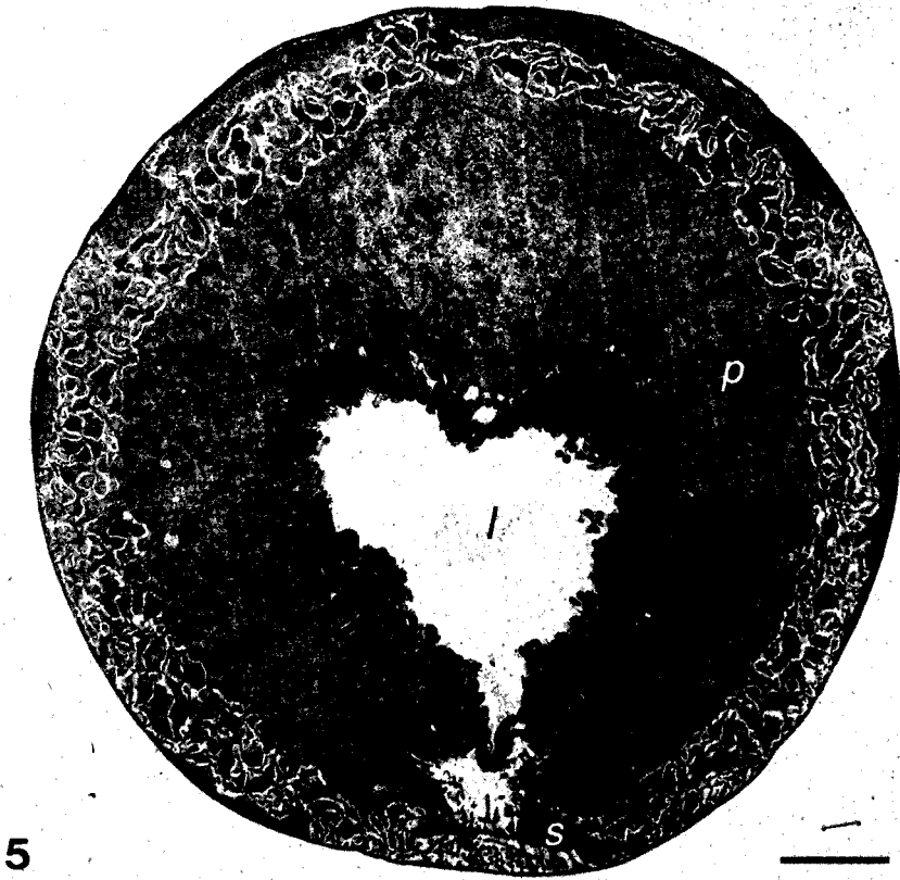
Fig. 5. An electron micrograph of a cross-section of a distal region of a non-lime gland tubule containing both a primary ( p ) and secondary ( s ) cell. l , lumen. Scale bar, 5 \mu m.
