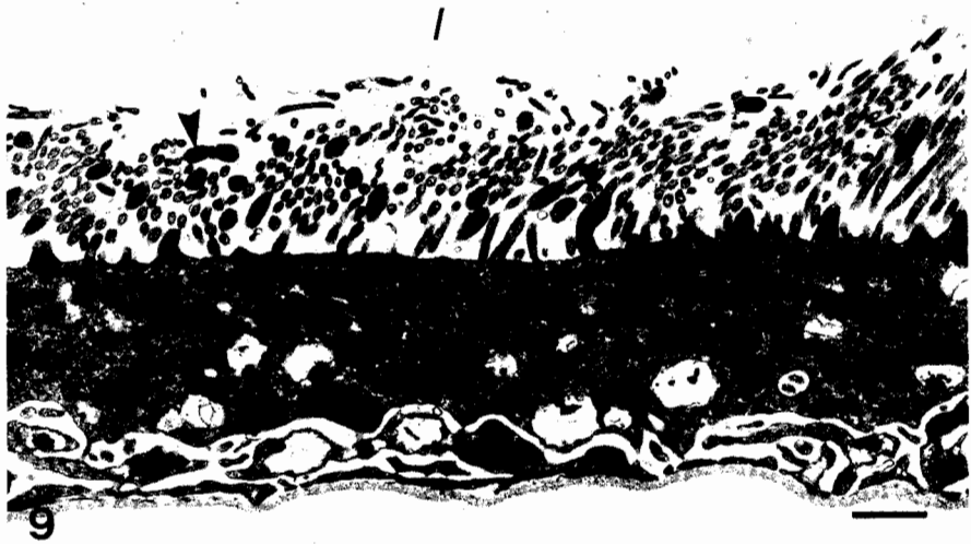
Fig. 9. An electron micrograph of the distal region of a lime gland tubule. Some microvilli in this region also contain mitochondria (arrowheads). l , lumen. Scale bar, 1 \mu m.
